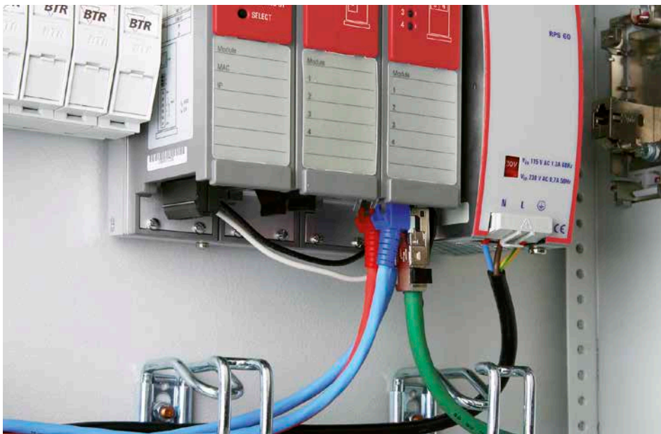
Fig. 5: Direct connection in the industry distributor
