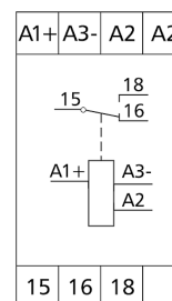
Raccordements
