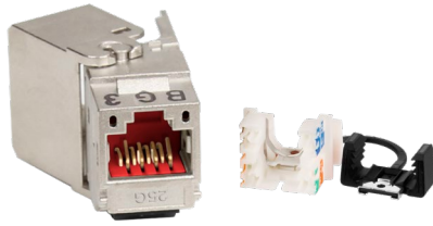
Keystone 130B21-25-E 180°
